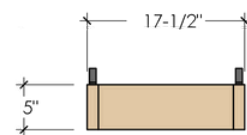
WOODEN LADDER
